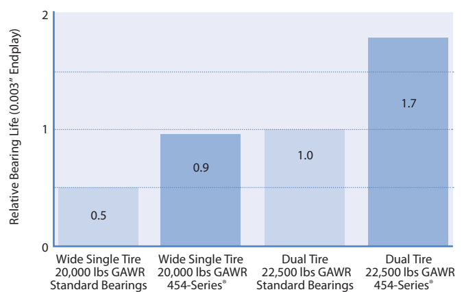
N-Trailer Predicted Wheel Bearing Fatigue Life
